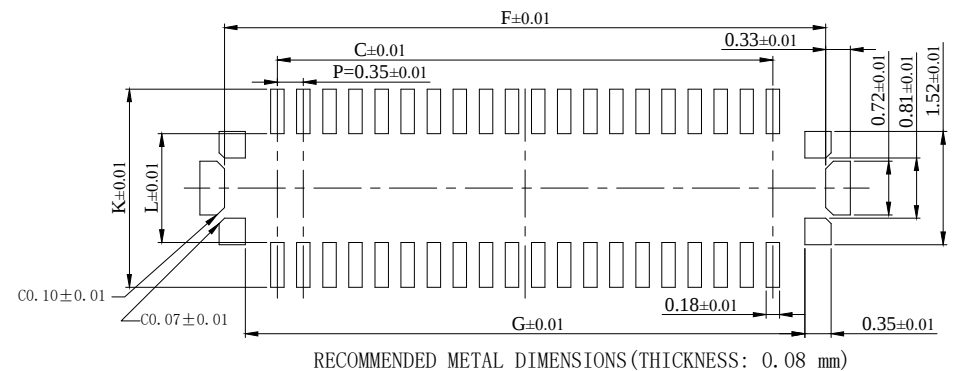
RECOMMENDED METAL DIMENSIONS (THICKNESS: 0.08 mm)
